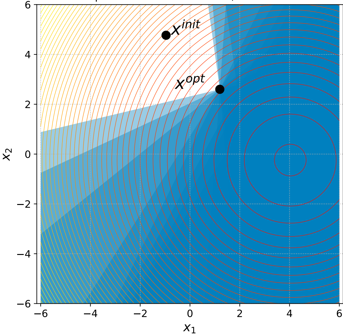
5 Sphere with 6+n constraints, instance=13
