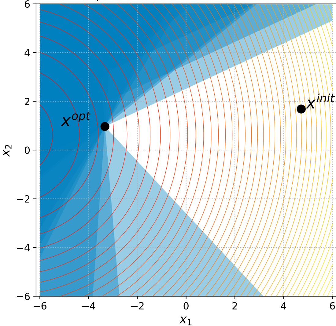
5 Sphere with 6+n constraints, instance=8
