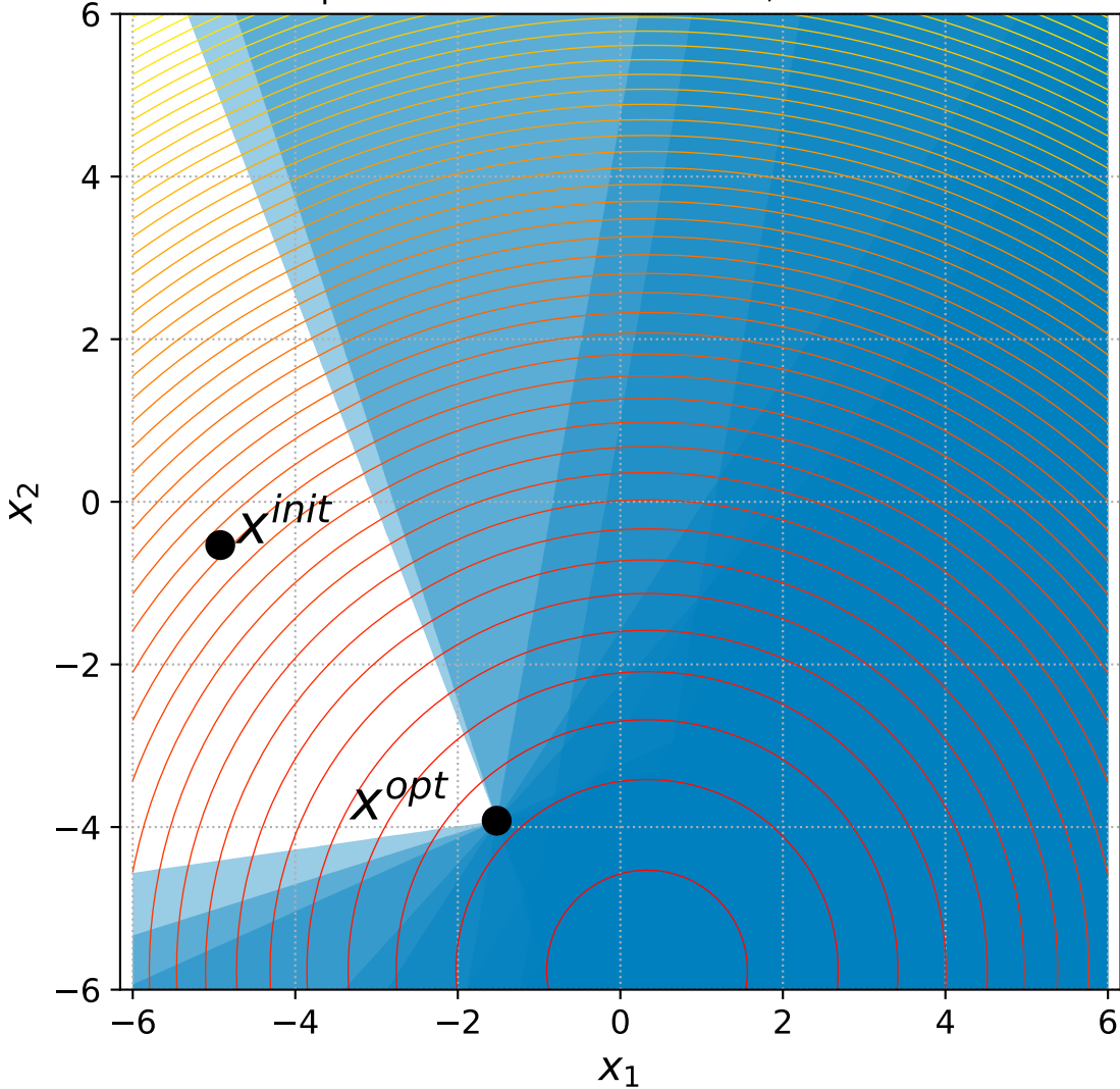
5 Sphere with 6+n constraints, instance=7
