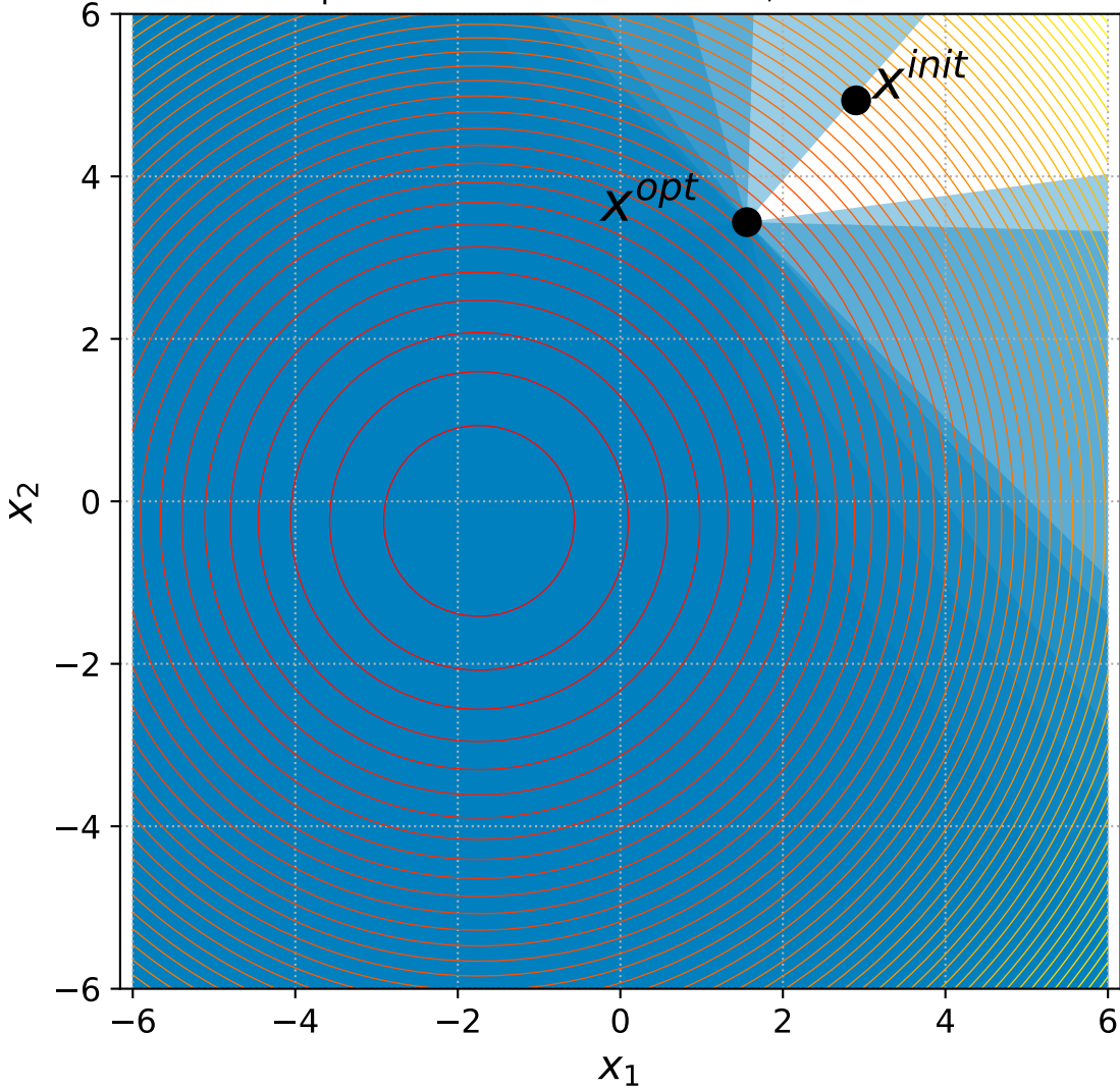
5 Sphere with 6+n constraints, instance=6
