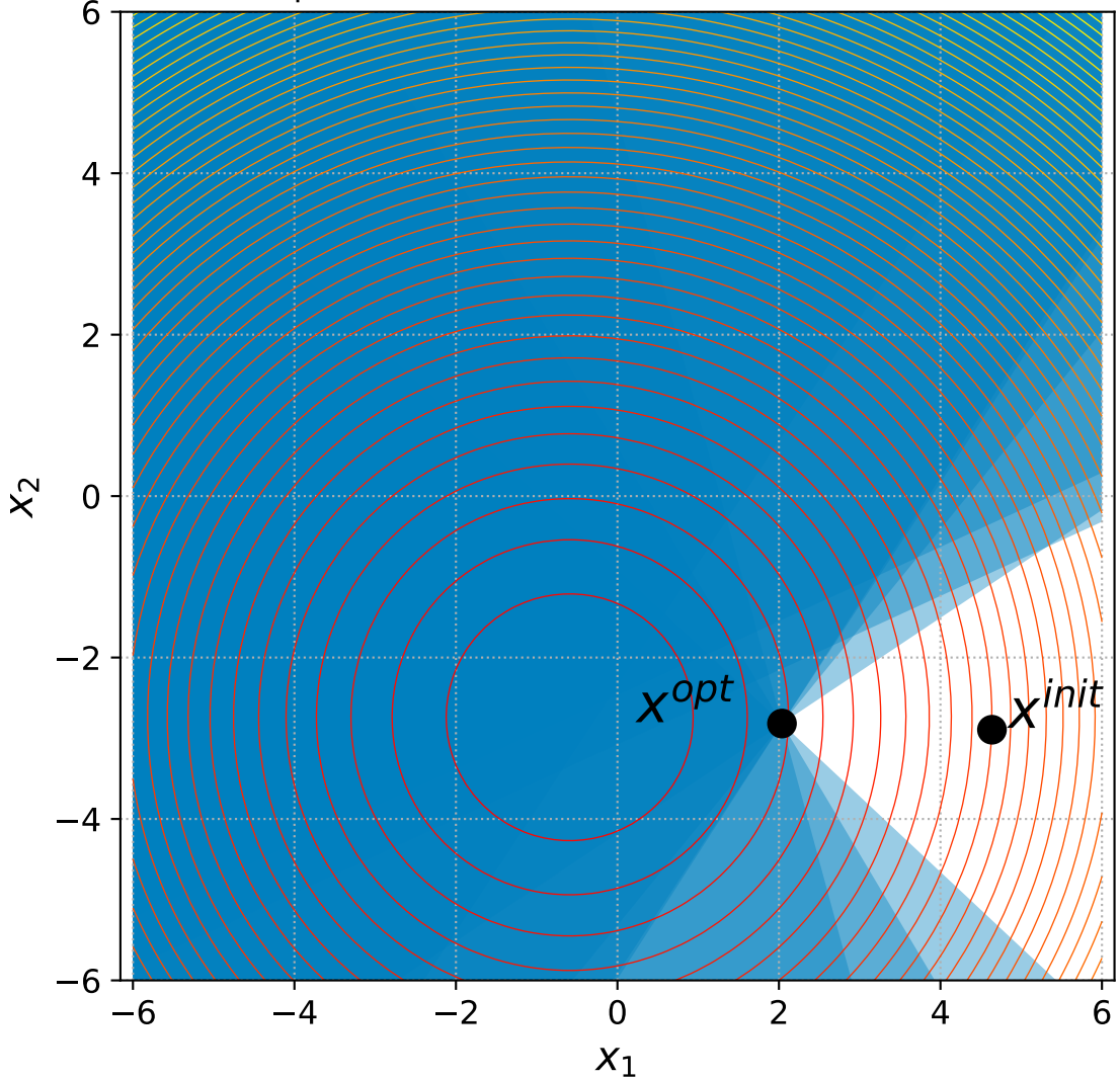
4 Sphere with 6+n/2 constraints, instance=15
