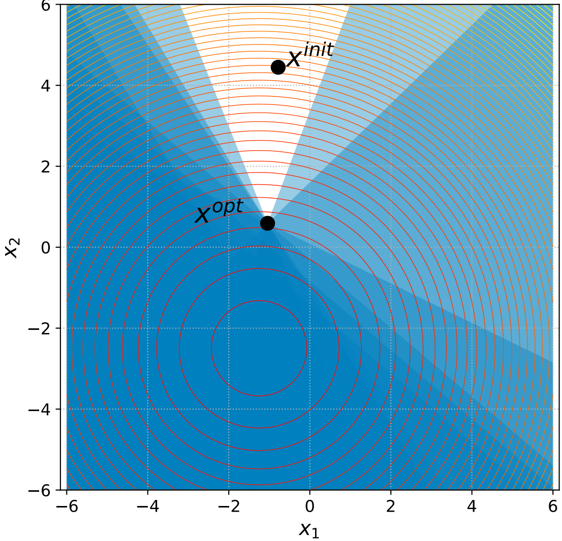
4 Sphere with 6+n/2 constraints, instance=14
