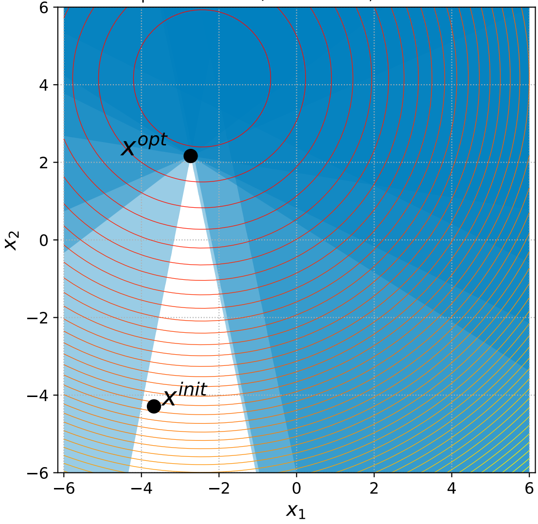
4 Sphere with 6+n/2 constraints, instance=12
