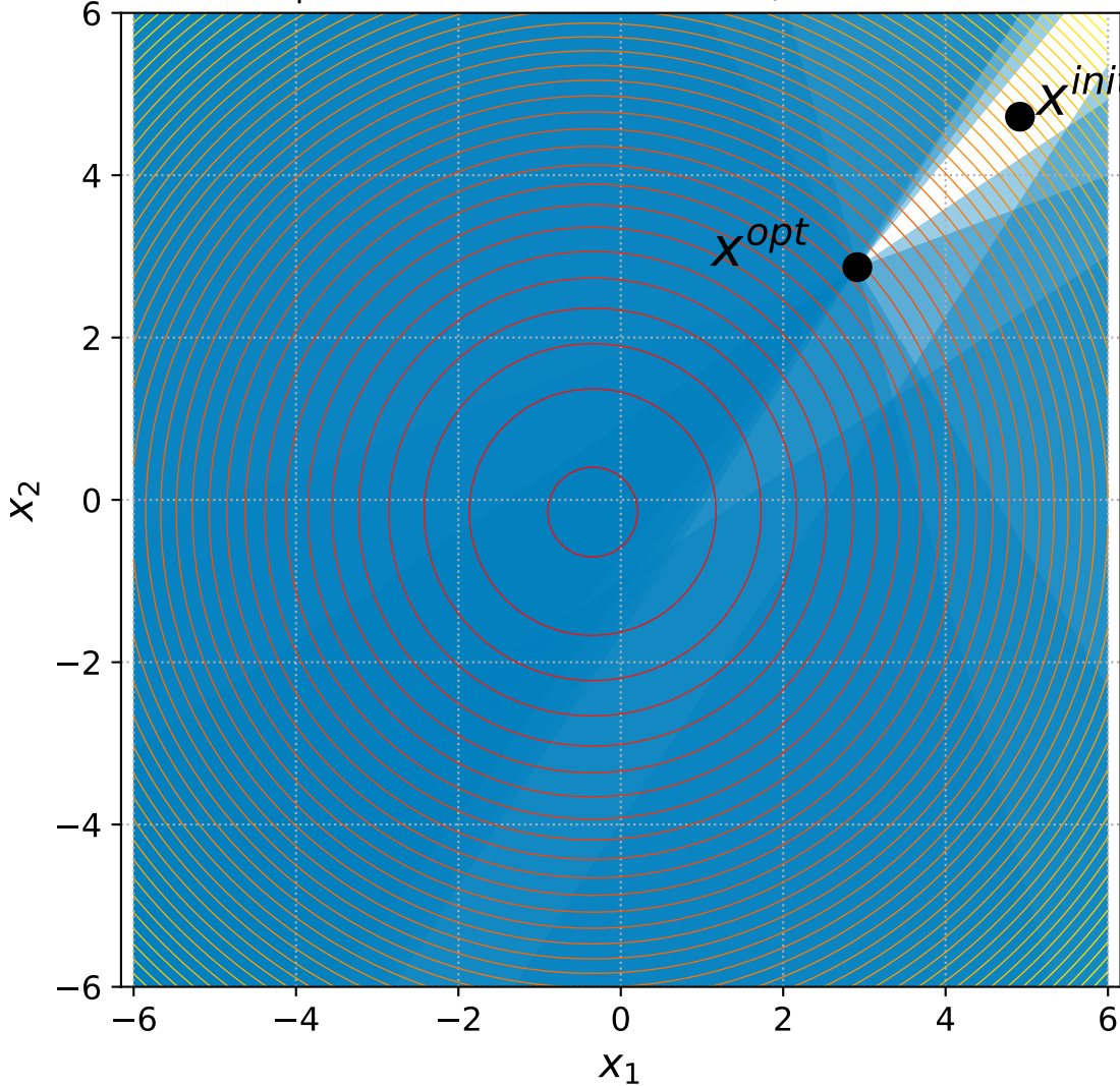
4 Sphere with 6+n/2 constraints, instance=10
