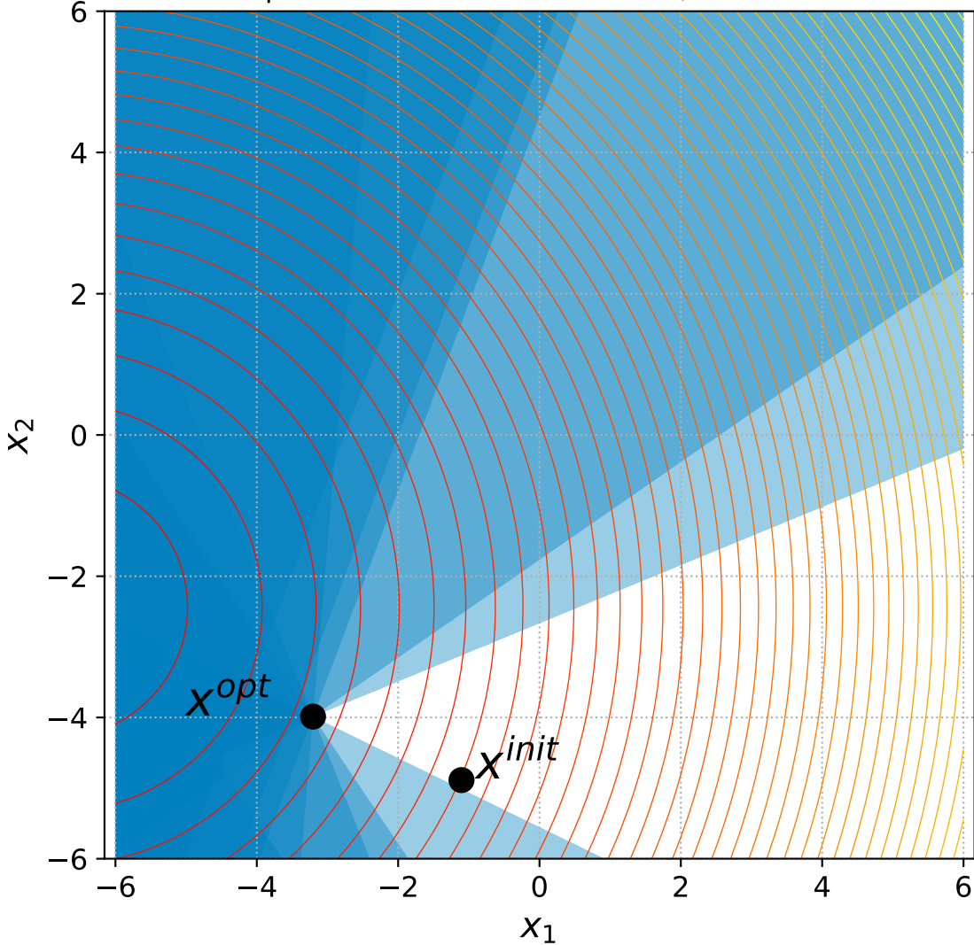
4 Sphere with 6+n/2 constraints, instance=9
