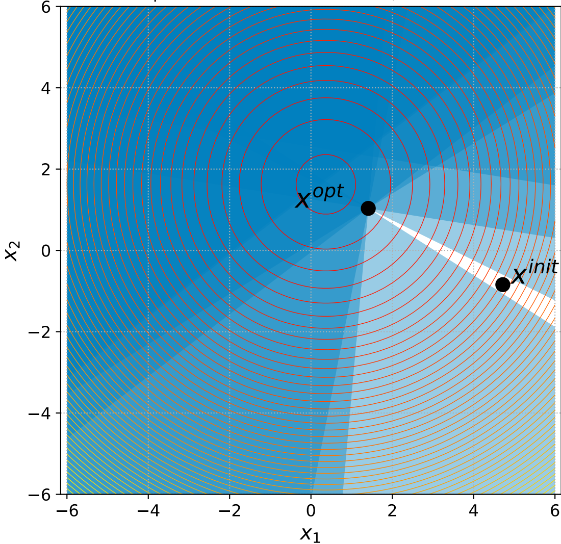
4 Sphere with 6+n/2 constraints, instance=7
