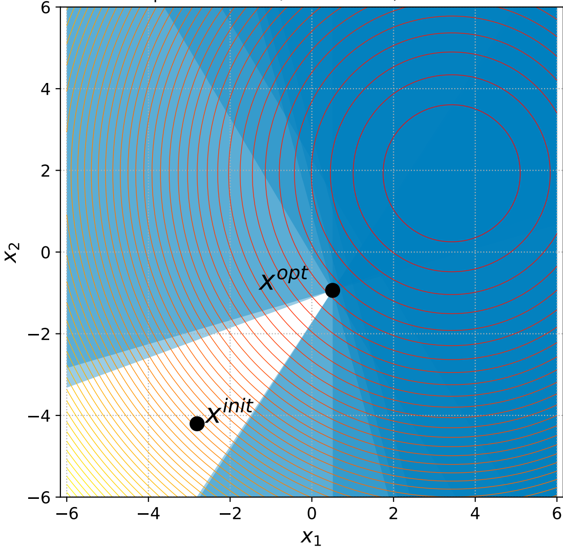
4 Sphere with 6+n/2 constraints, instance=5
