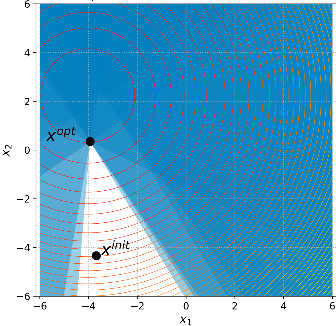
4 Sphere with 6+n/2 constraints, instance=4
