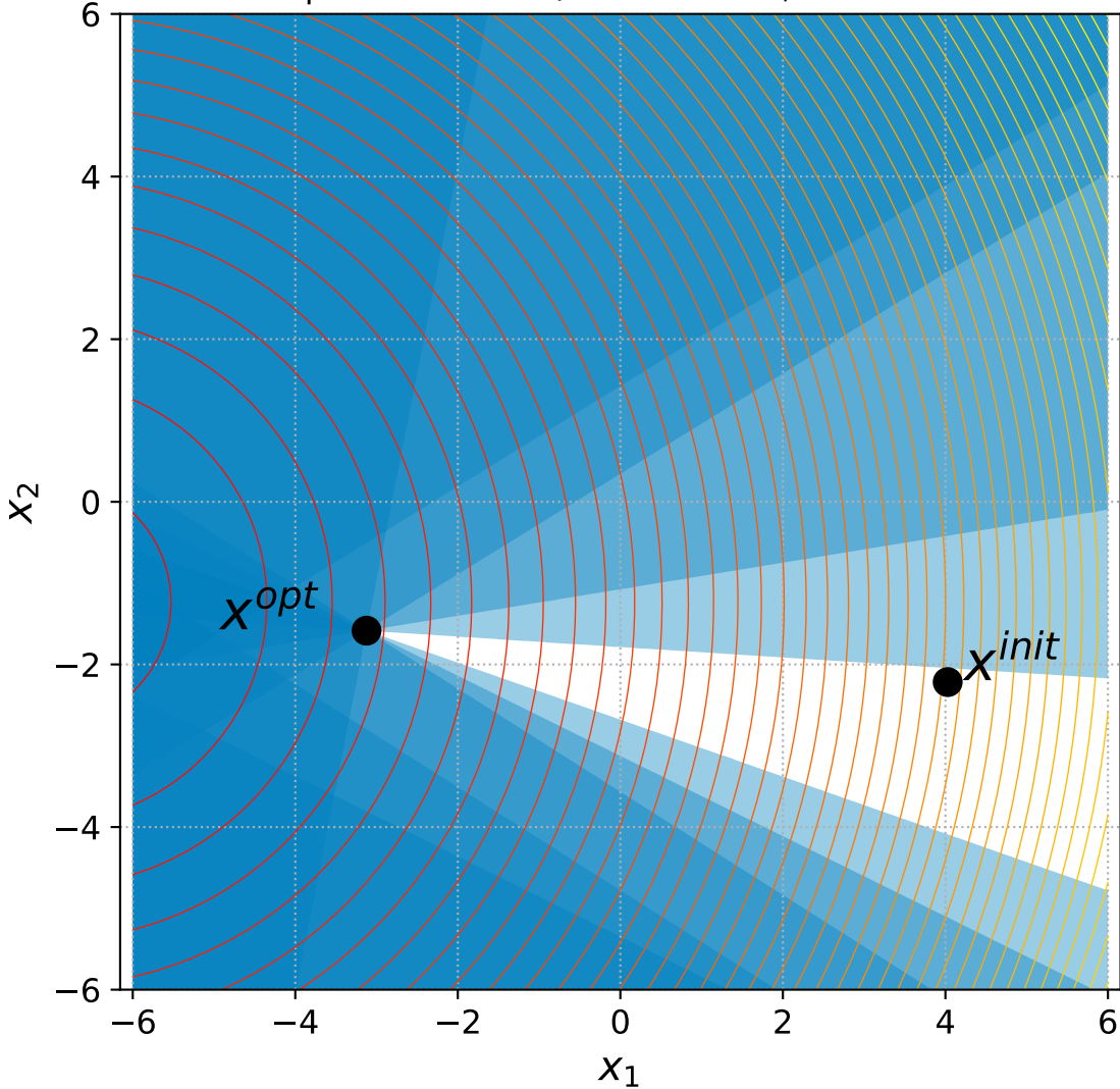
4 Sphere with 6+n/2 constraints, instance=2
