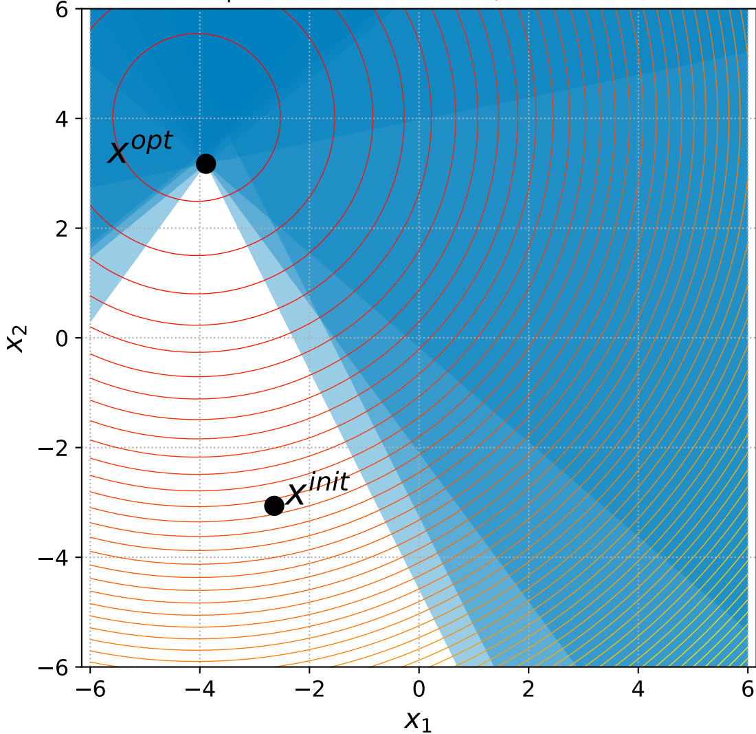
3 Sphere with 6 constraints, instance=15
