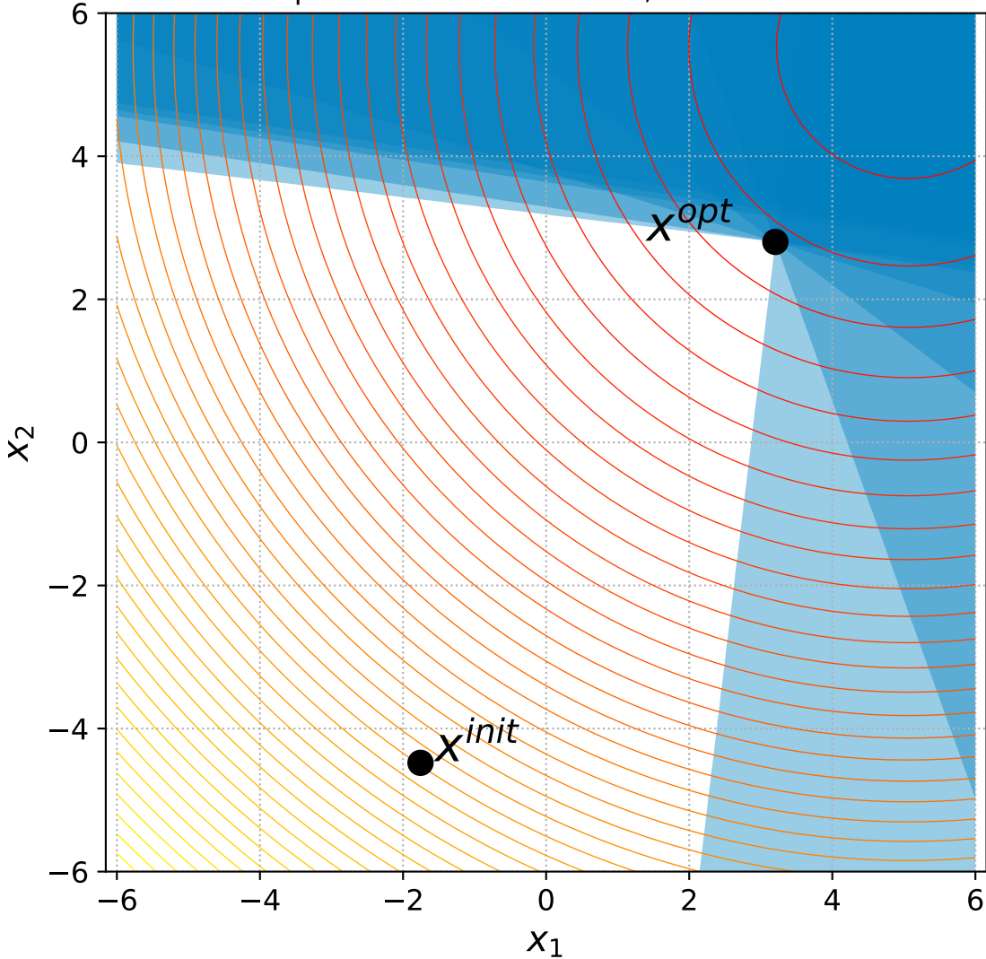
3 Sphere with 6 constraints, instance=14
