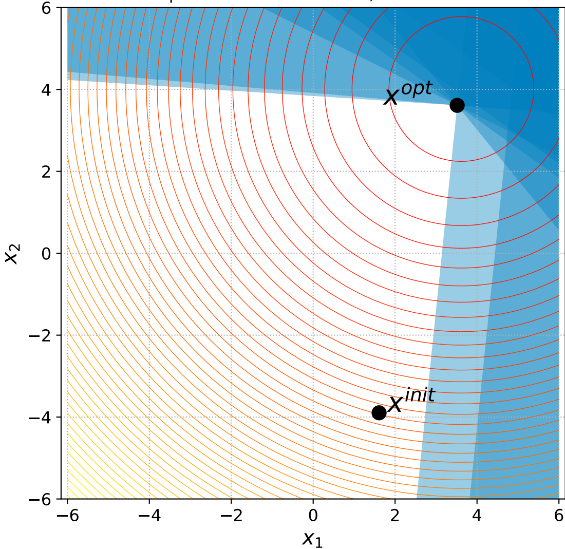
3 Sphere with 6 constraints, instance=12
