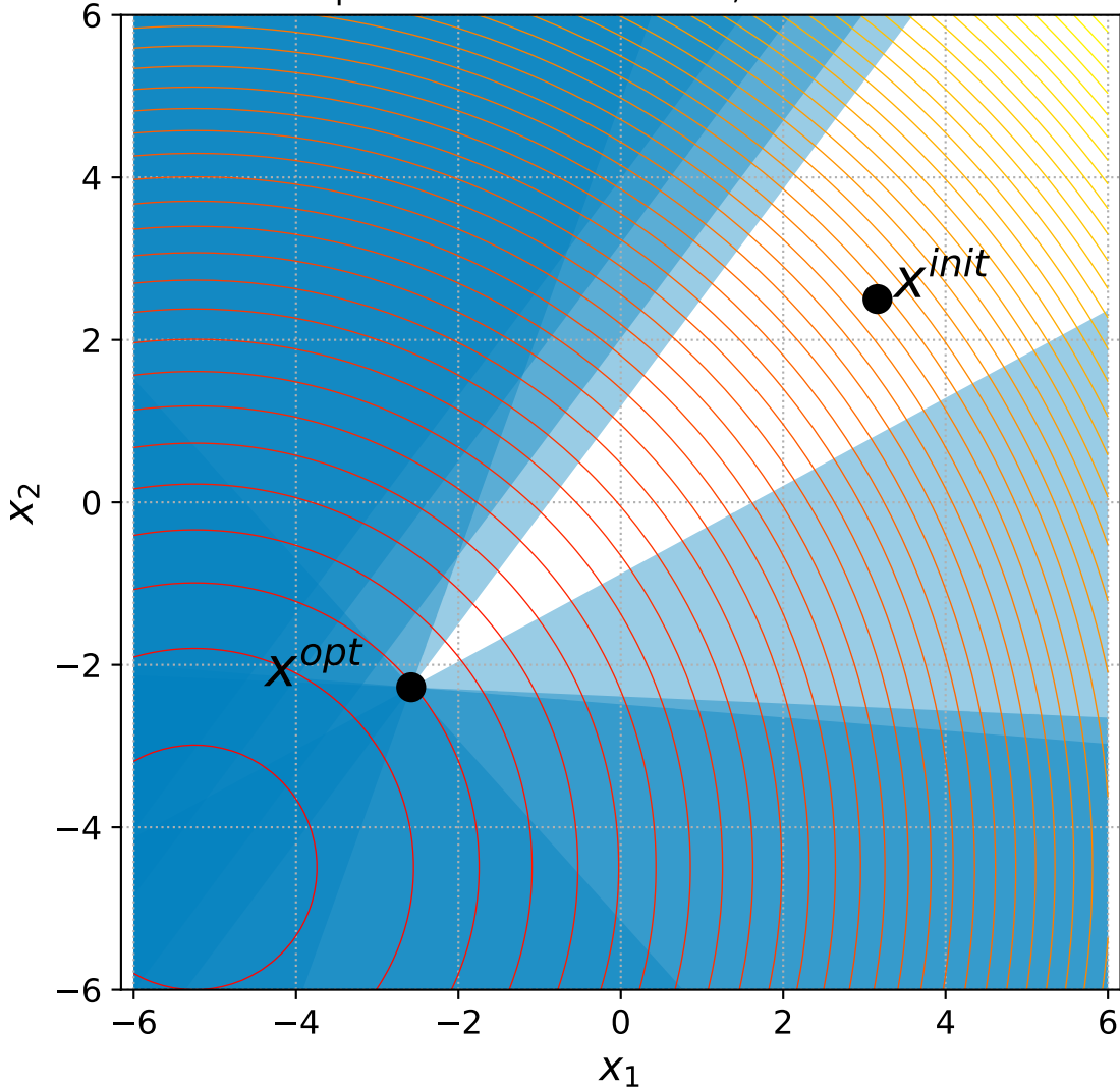
3 Sphere with 6 constraints, instance=11
