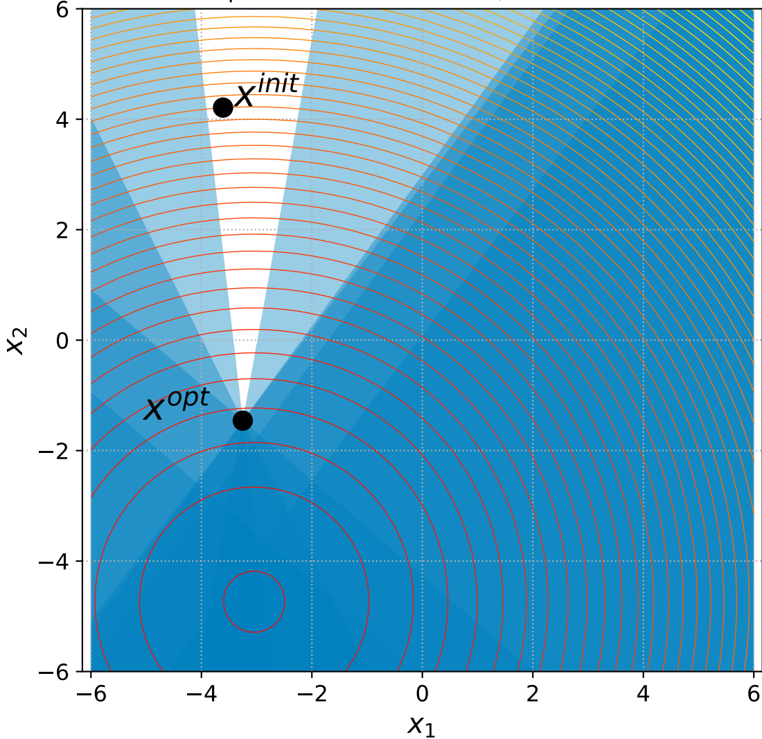
3 Sphere with 6 constraints, instance=10
