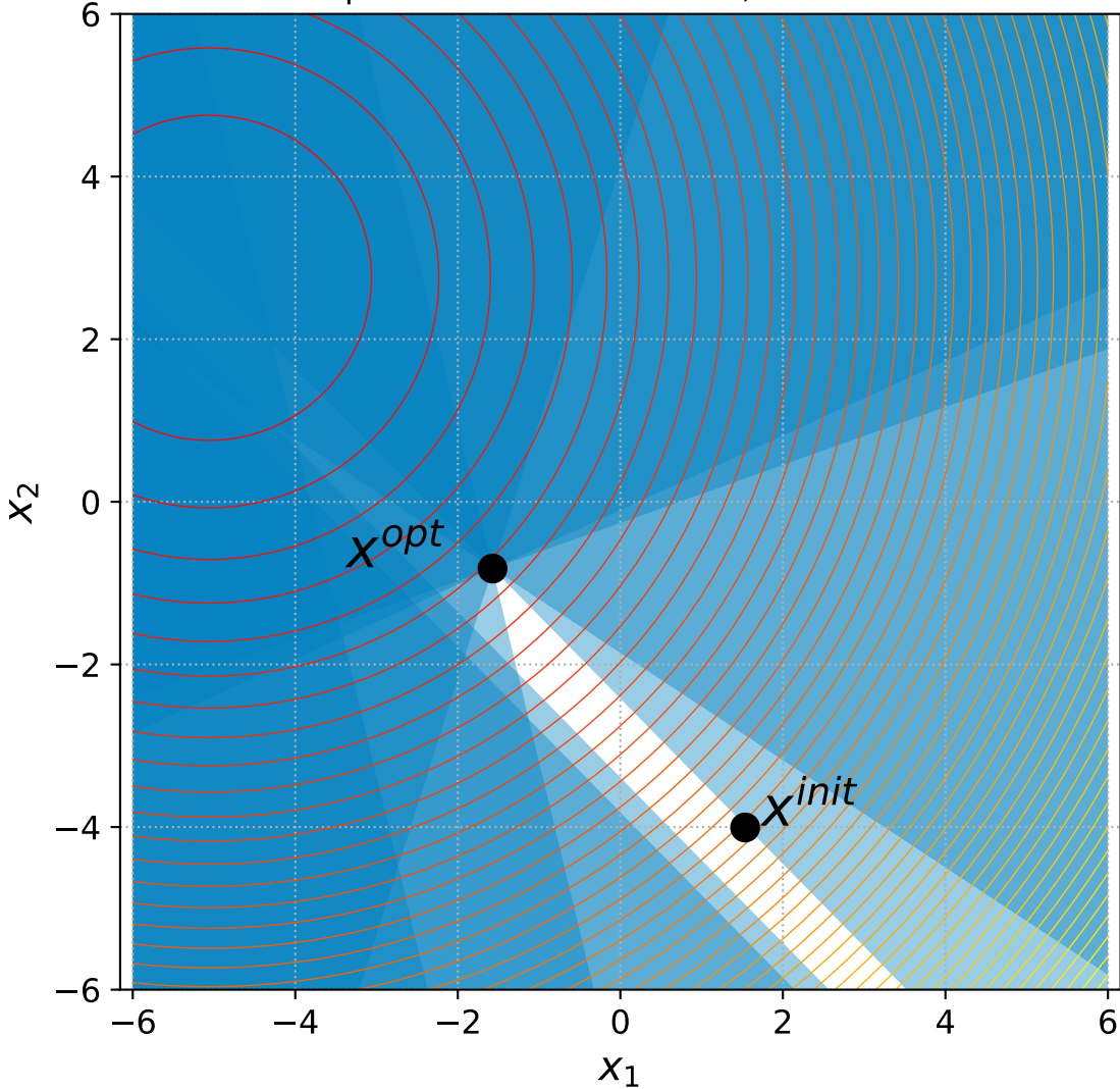
3 Sphere with 6 constraints, instance=8
