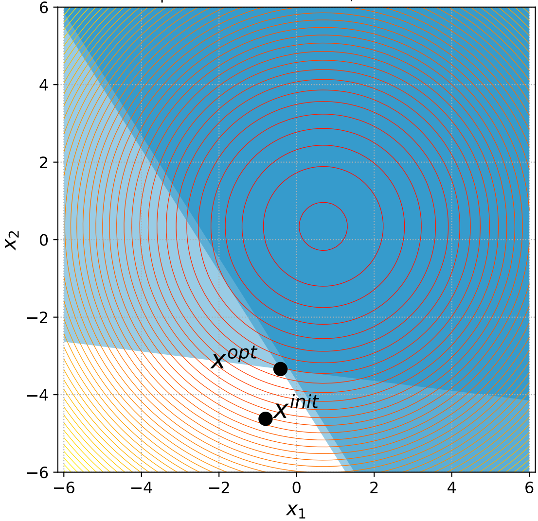
2 Sphere with 2 constraints, instance=14
