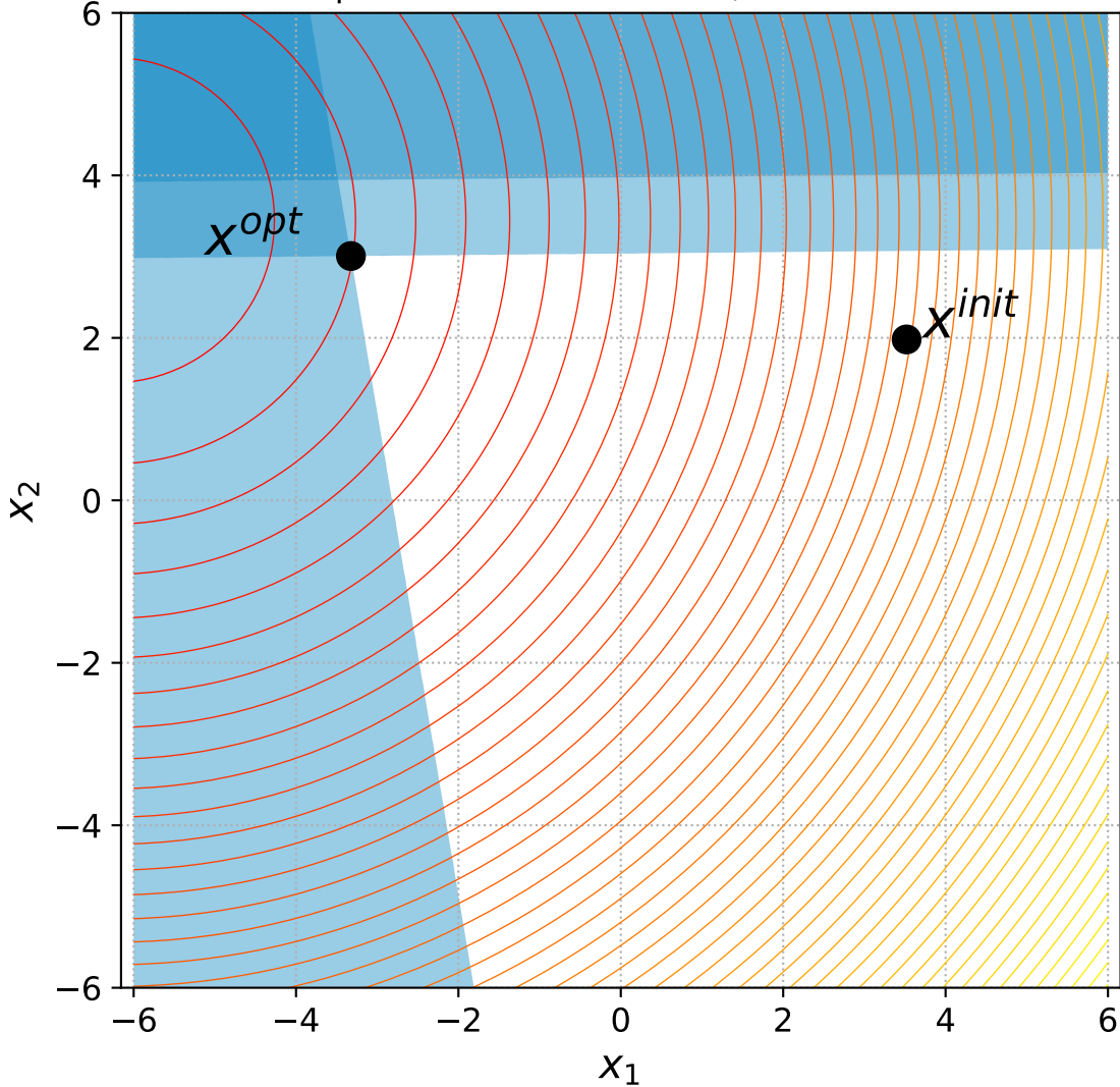
2 Sphere with 2 constraints, instance=13
