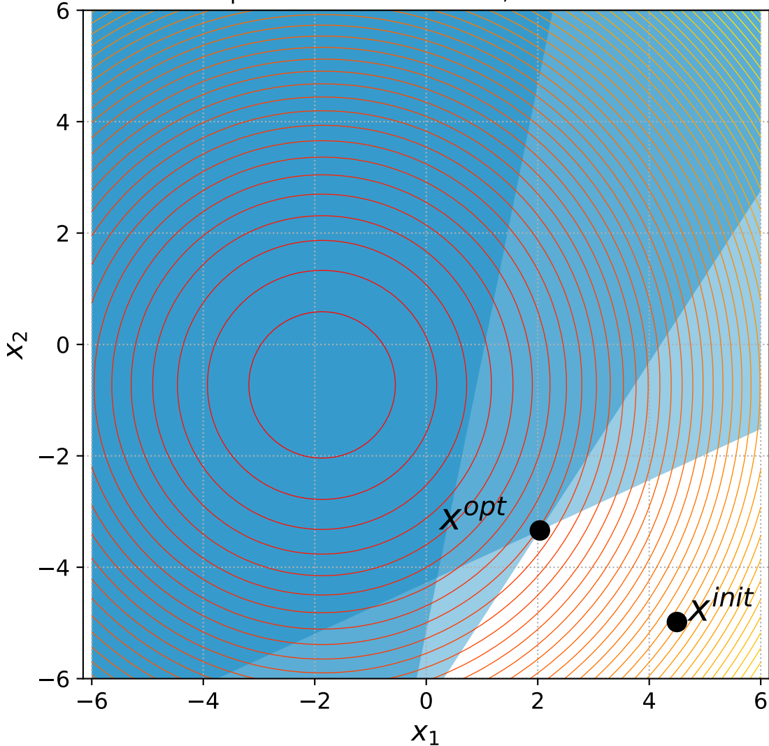
2 Sphere with 2 constraints, instance=12
