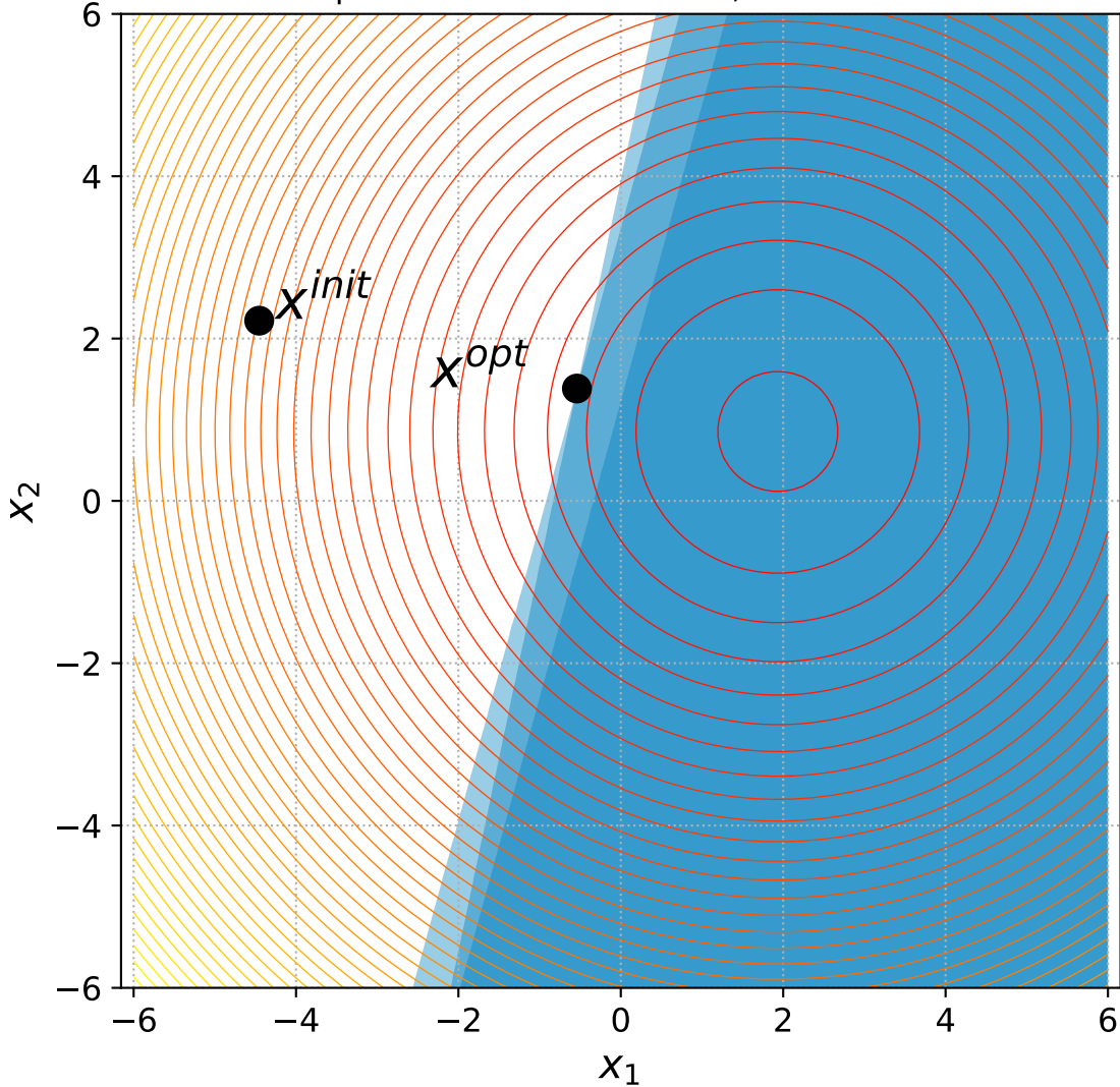
2 Sphere with 2 constraints, instance=10
