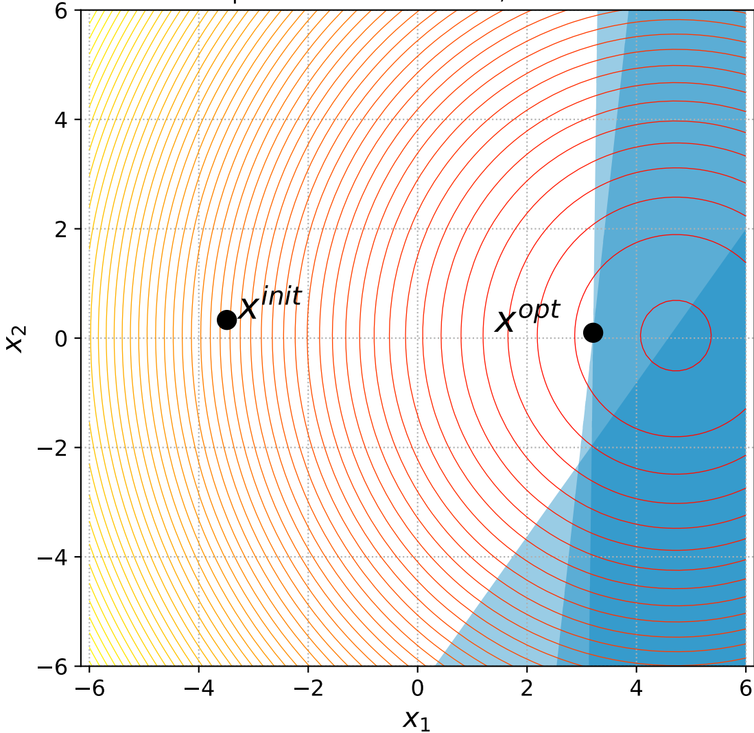
2 Sphere with 2 constraints, instance=9
