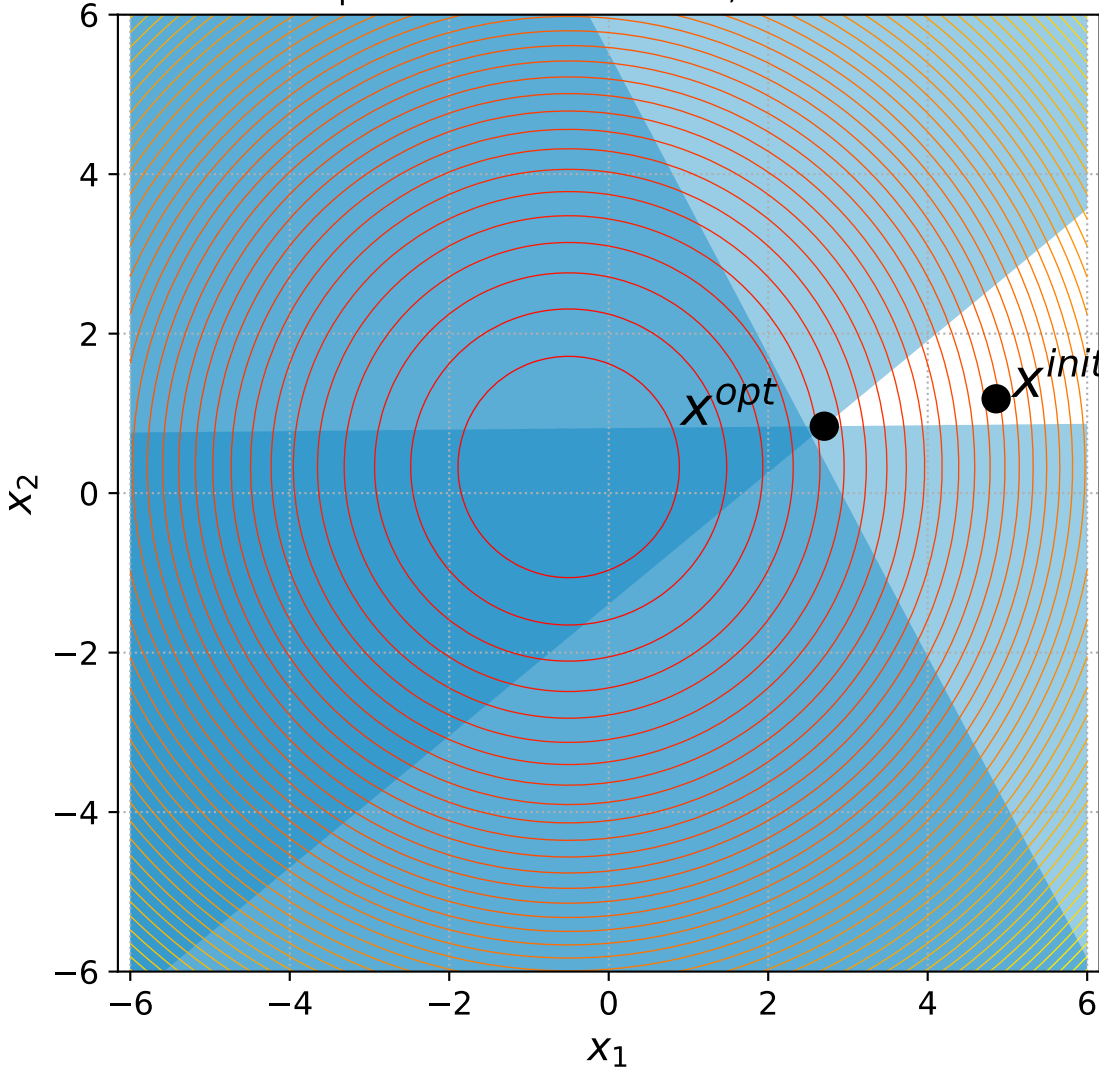
2 Sphere with 2 constraints, instance=8
