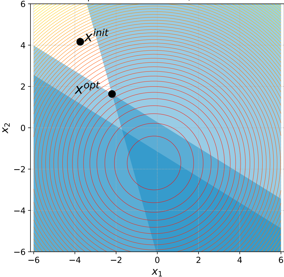
2 Sphere with 2 constraints, instance=6
