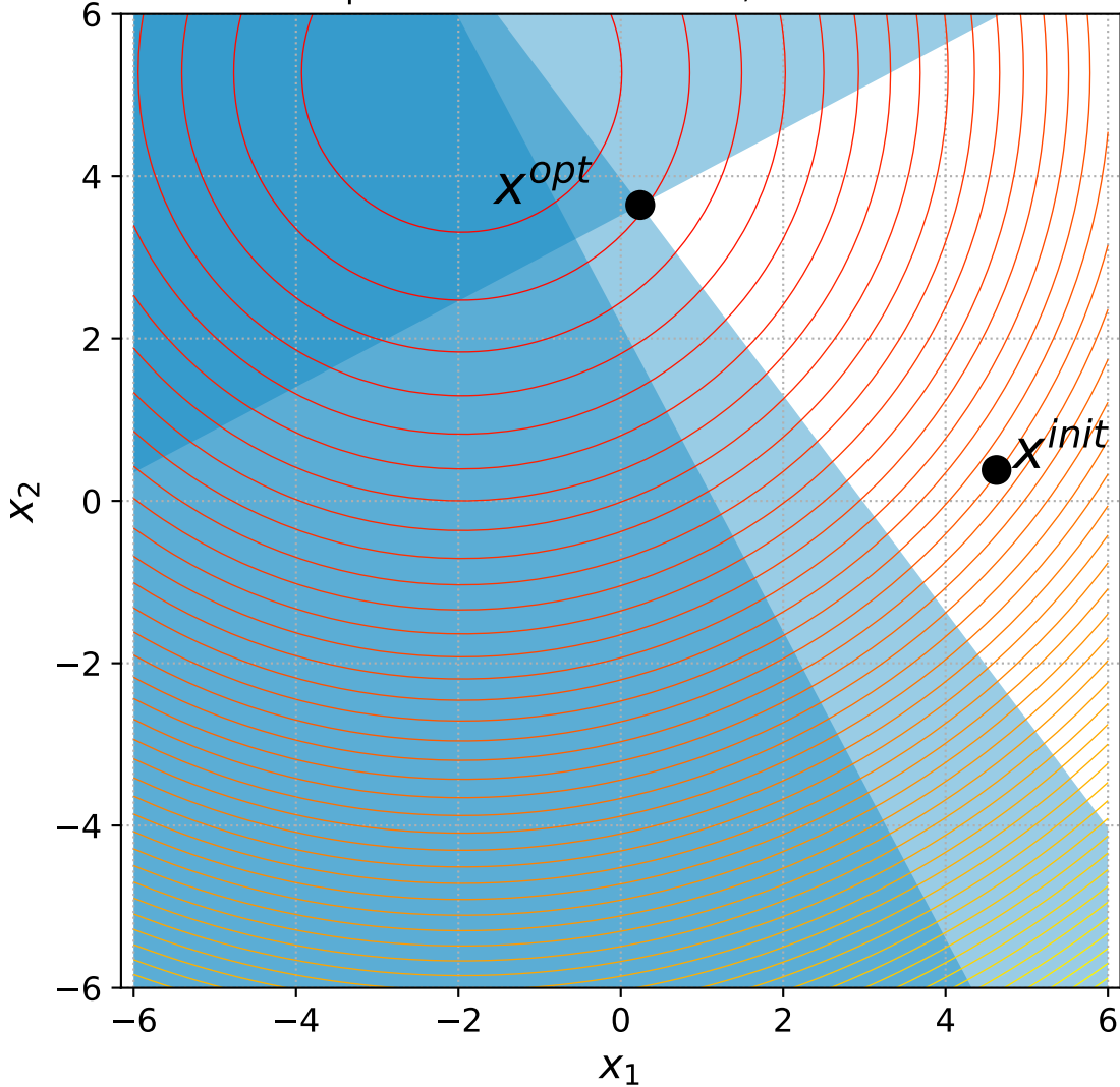
2 Sphere with 2 constraints, instance=3
