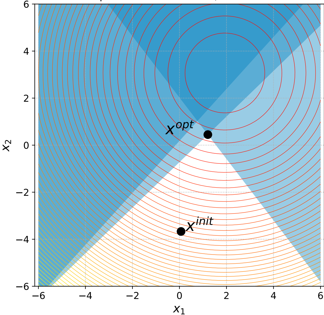
2 Sphere with 2 constraints, instance=1
