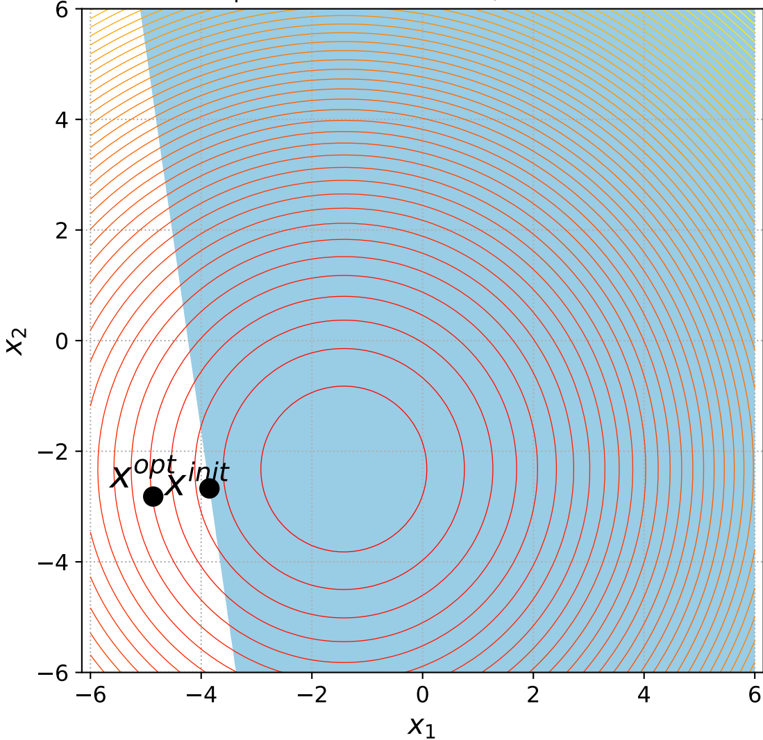
1 Sphere with 1 constraint, instance=15
