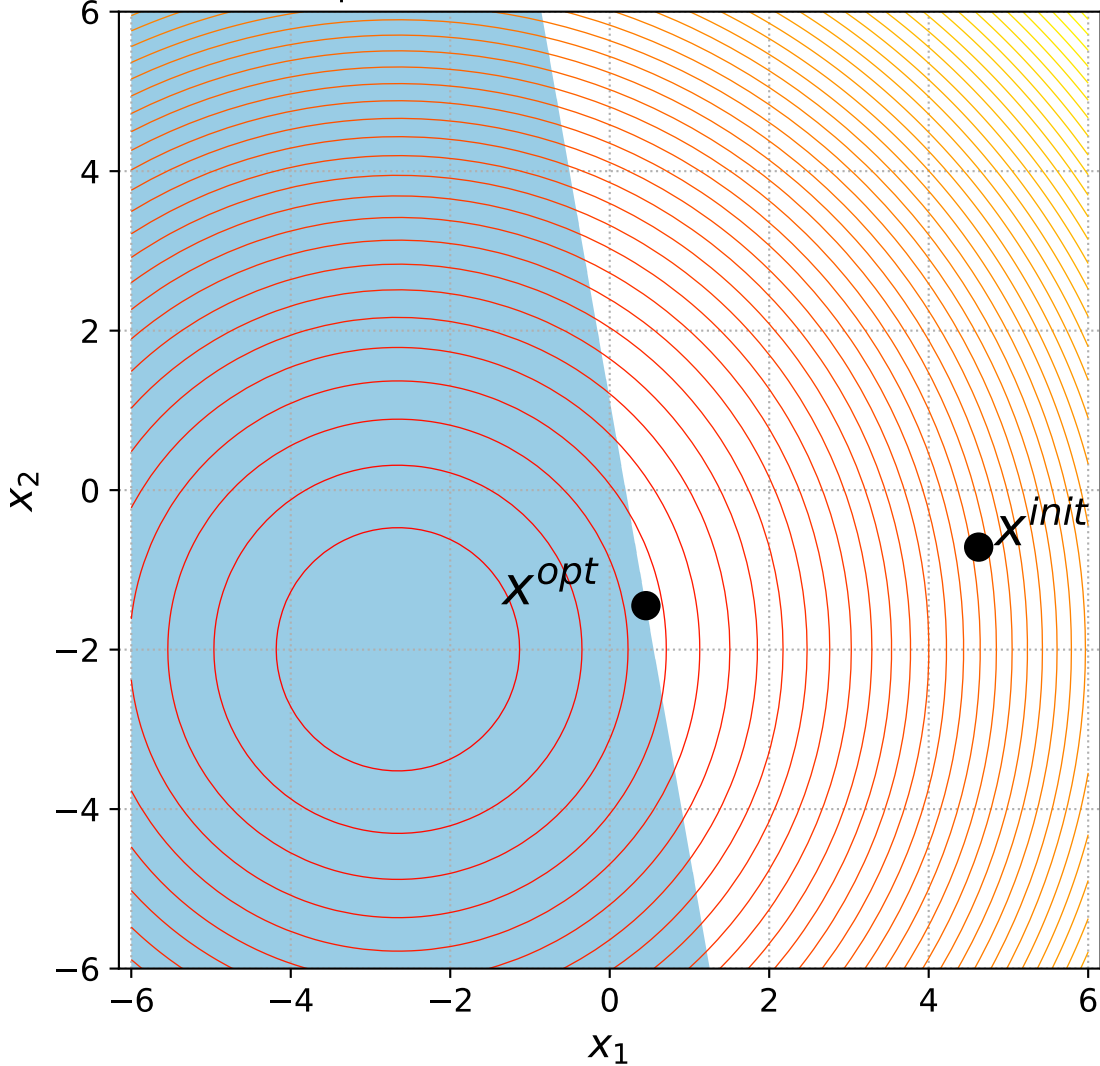
1 Sphere with 1 constraint, instance=14
