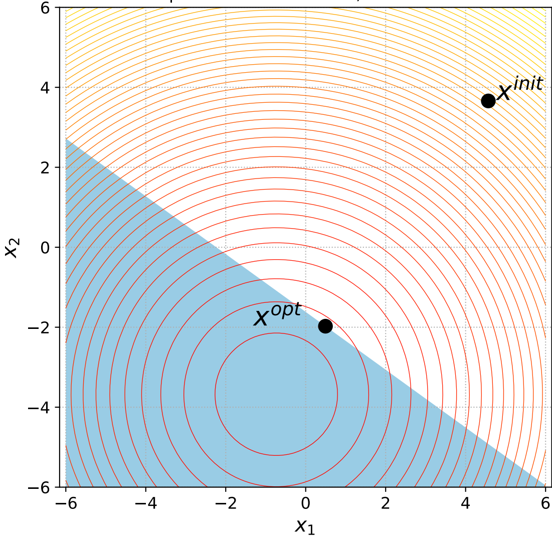
1 Sphere with 1 constraint, instance=10
