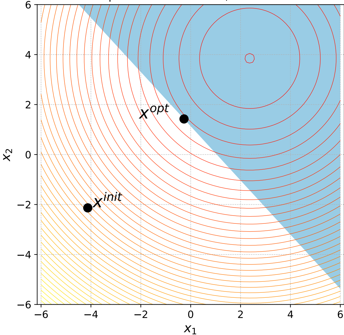
1 Sphere with 1 constraint, instance=4
